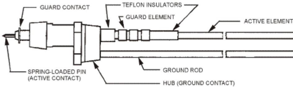
Figure 1-4 Standard L870 Probe, Descriptive Drawing
