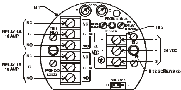
Figure 3-5 Electrical Connections – 24Vdc Units
