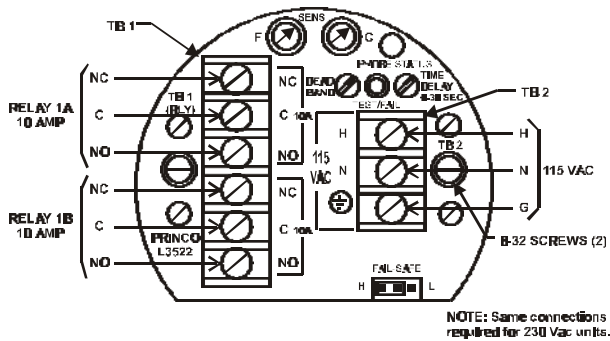
Figure 3-4 Electrical Connections – 115Vac & 230Vac Units
